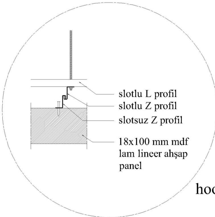
Drawing 3: Wood Linear Ceiling Detail
