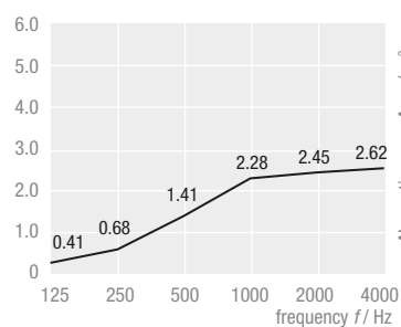
THERMATEX® Sonic element square 1200 x 1200 mm, Assembly height 300 mm
