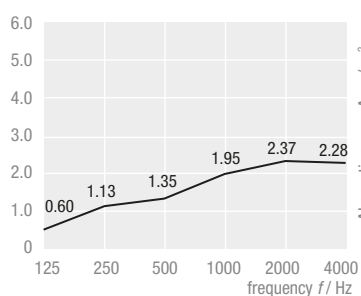
THERMATEX® Sonic modern square 1200 x 1200 mm, Assembly height 300 mm
