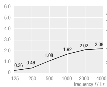
THERMATEX® Sonic element round Ø 1200 mm, Assembly height 300 mm
