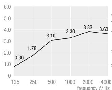
THERMATEX® Sonic modern rectangular 1200 x 2400 mm, Assembly height 150 mm
