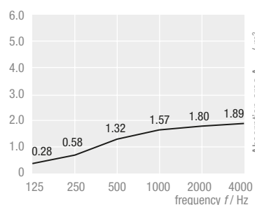
THERMATEX® Sonic element round Ø 1200 mm, Assembly height 150 mm
