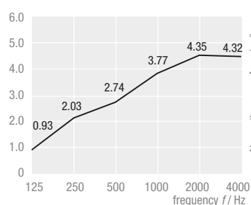
THERMATEX® Sonic modern rectangular 1200 x 2400 mm, Assembly height 300 mm
