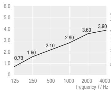
THERMATEX® Sonic arc 1180 x 1910 mm, Assembly height 300 mm
