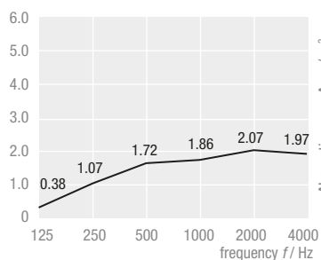
THERMATEX® Sonic modern square 1200 x 1200 mm, Assembly height 150 mm
