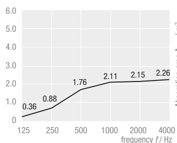
THERMATEX® Sonic element square 1200 x 1200 mm, Assembly height 150 mm
