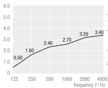
THERMATEX® Sonic arc 1180 x 1910 mm, Assembly height 150 mm
